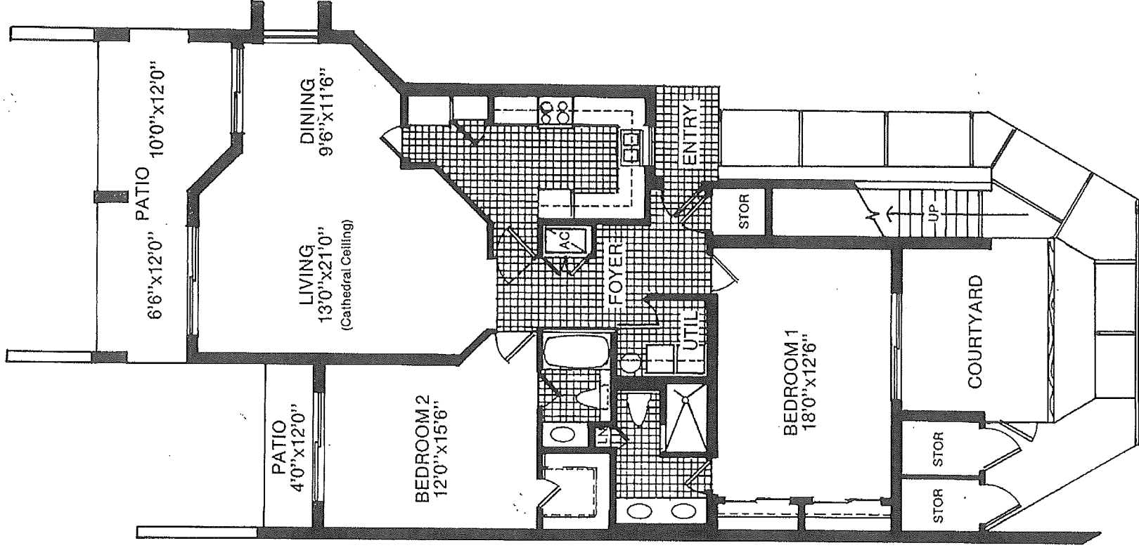
Courtyard Apartment FIRST FLOOR PLAN
